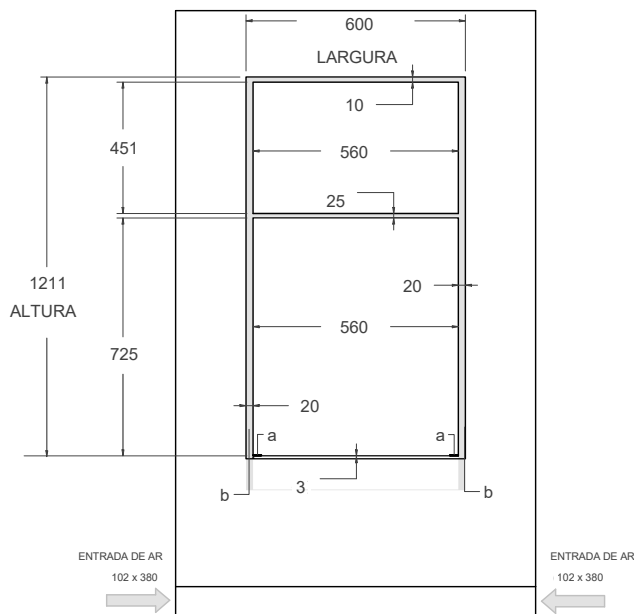
VISTA FRONTAL
